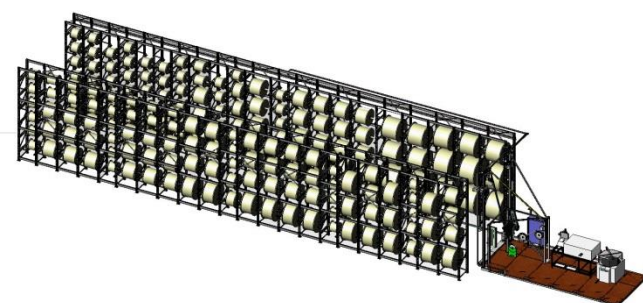
Semi-automatic reel storage system „3 in 1“ with powered platform
